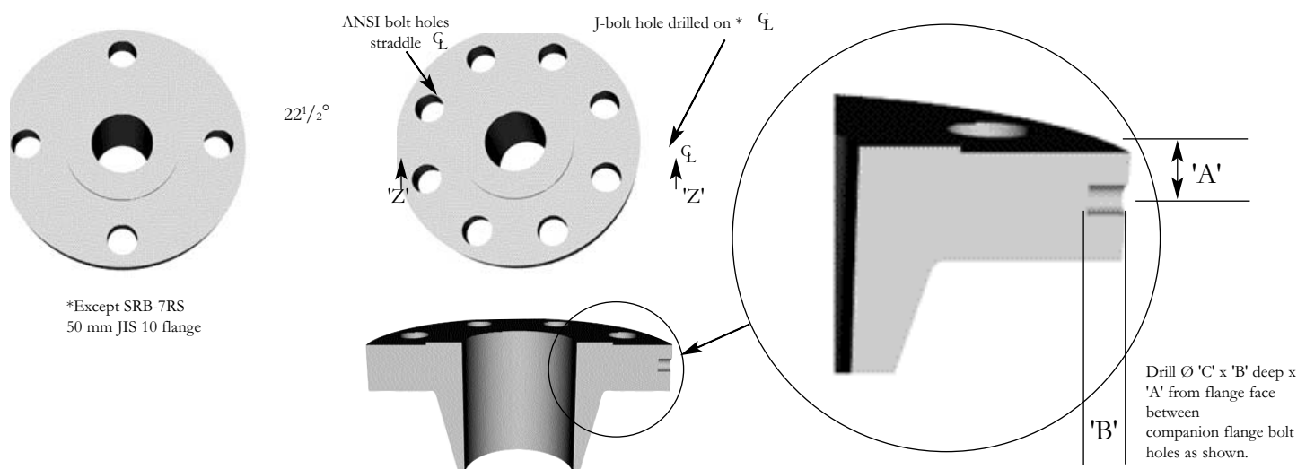
Figure 1: Inlet Companion Flange Drilling to Accept J-Bolt
